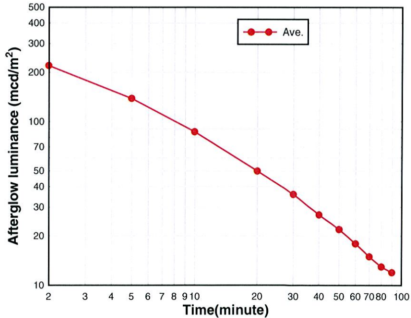
Fig. Afterglow Luminance of Ecoglo S20 sign material Excitation:WFL FL15W(4200K) 100lx, 5min.
